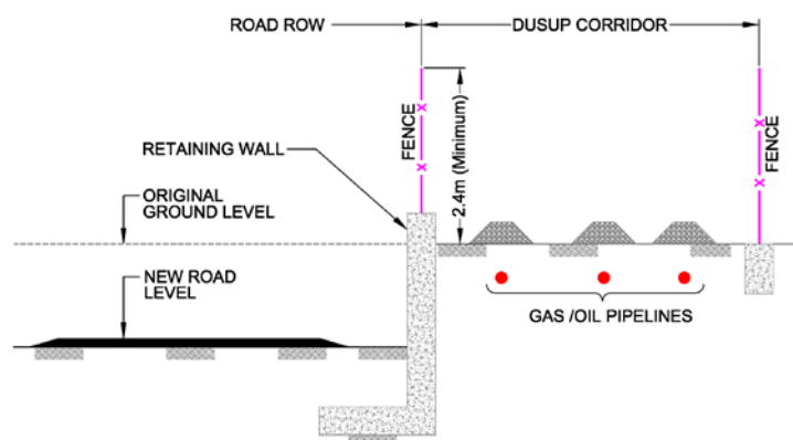
RETAINING WALL AT DUSUP CORRIDOR
